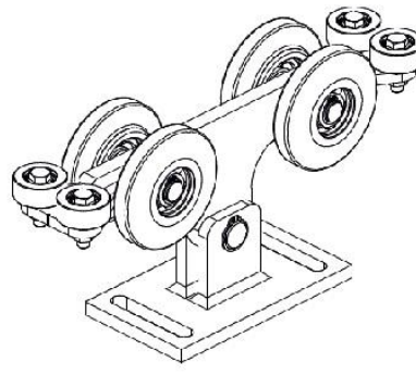
Rollenset 5-6m
