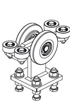
Rollenset 2-4m
