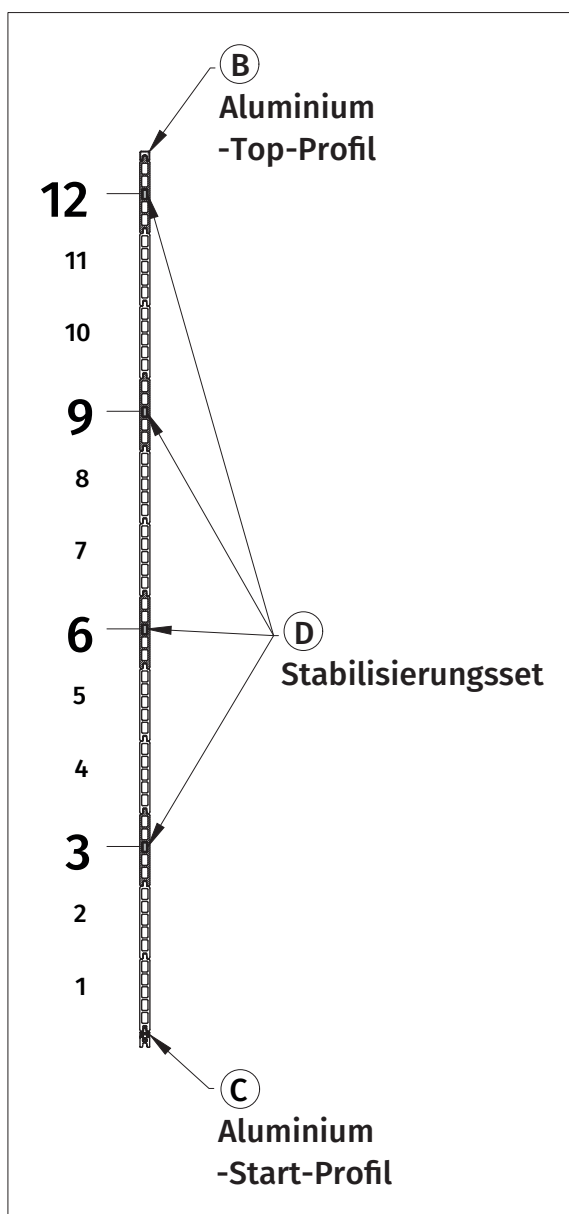
Detail 2.3-1
