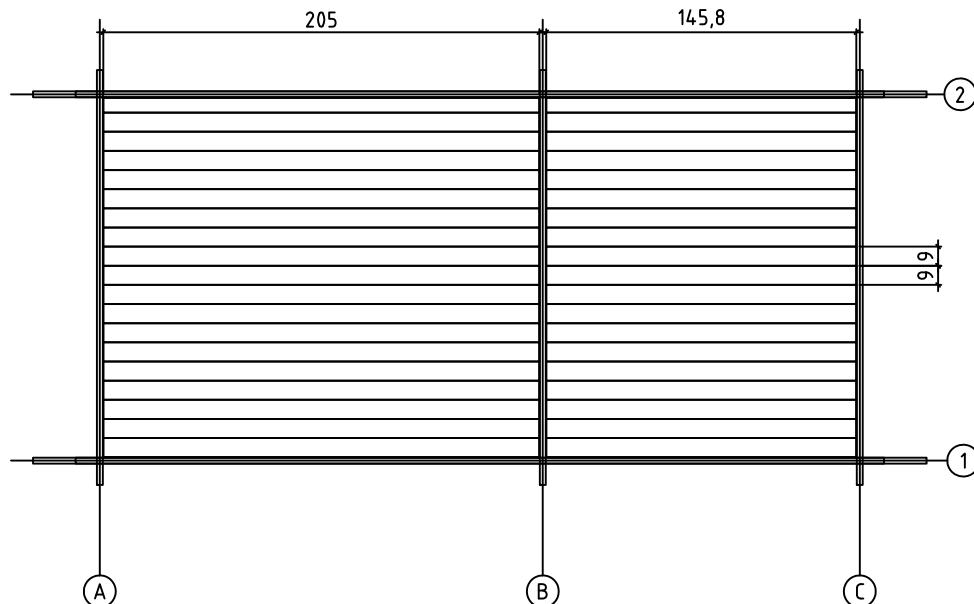
FLOOR BOARDS -FUSSBODENBRETTER - PLAN POSE PLANCHER
